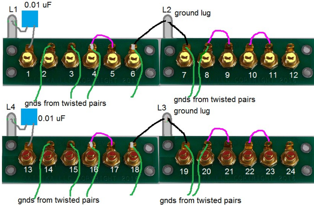
Figure 4-Wiring Grounds, lugs, and capacitors on the new jack fields
