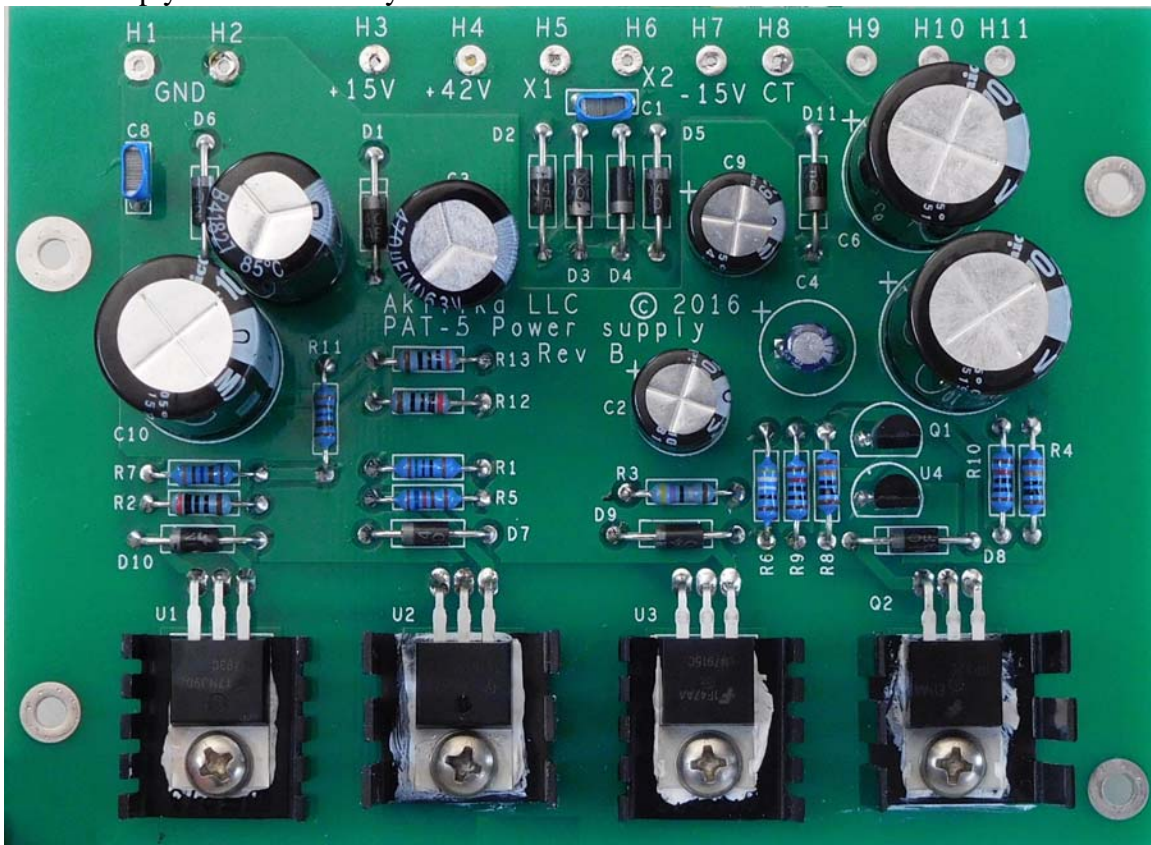
Figure 1-Assembled PAT-5 Power Supply. Note that U2 and Q2 get tall heatsinks
