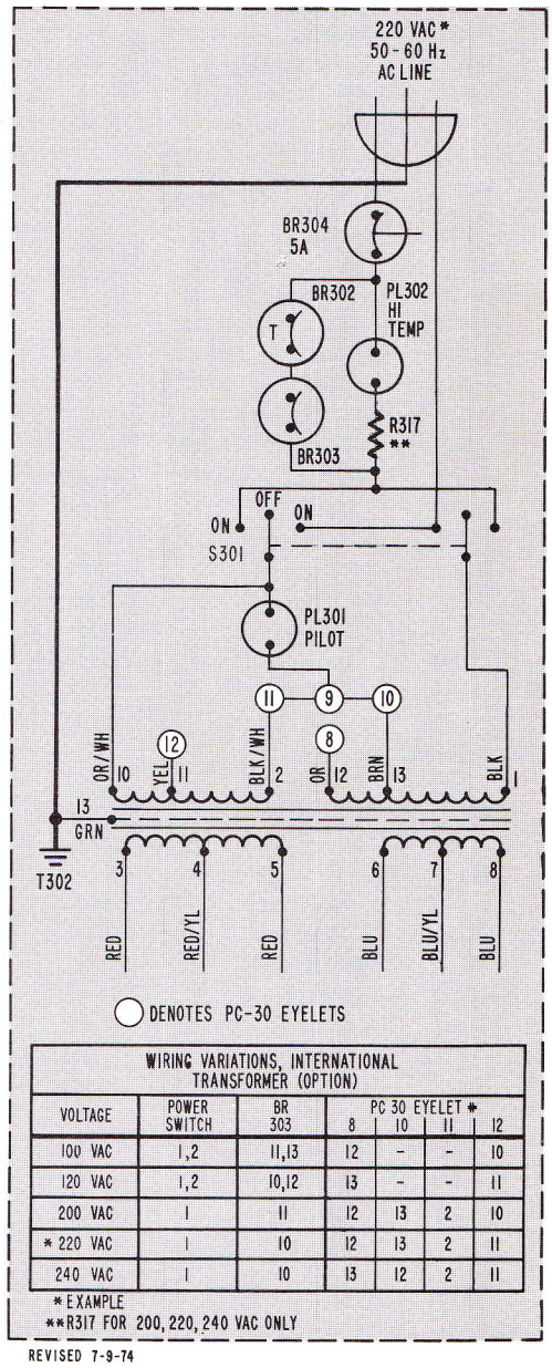
SCHEMATIC DIAGRAM ©1973 DYNACO INC.
